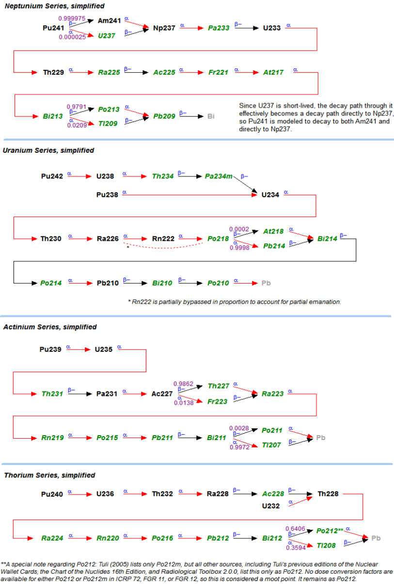
Figure 12. Principal decay chains for the four actinide series. Radionuclides in black are included in the fate and transport model, and those in green are considered only in the dose model.
