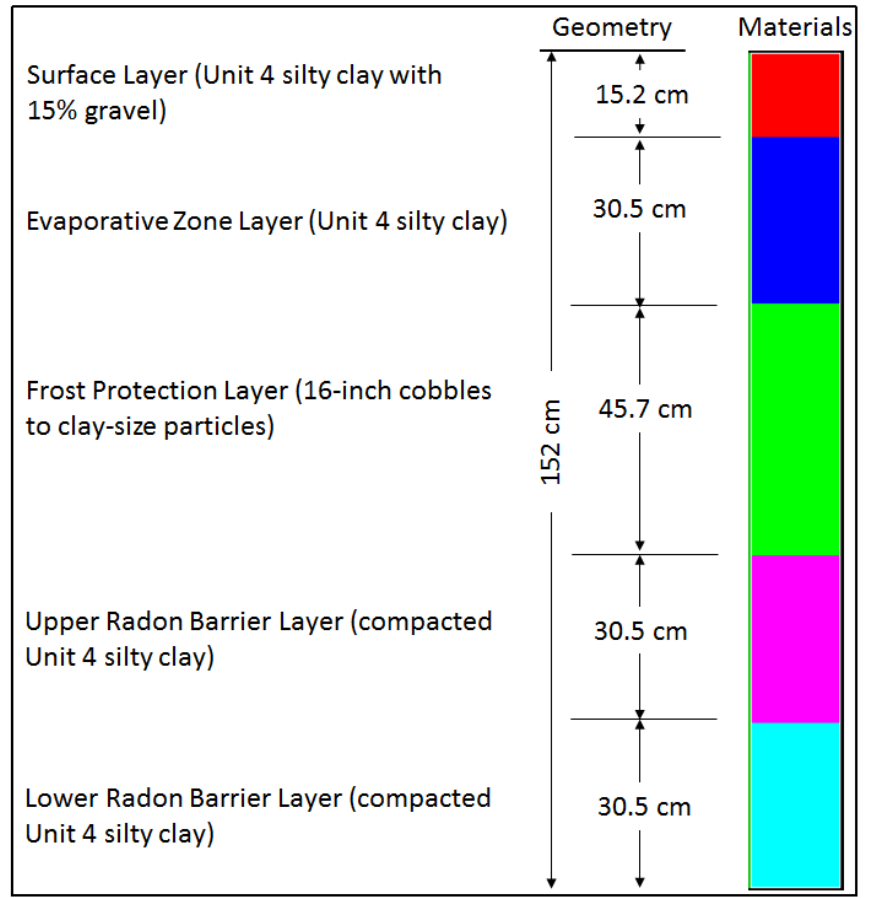
Figure 7. Evapotranspiration (ET) cover system.—
