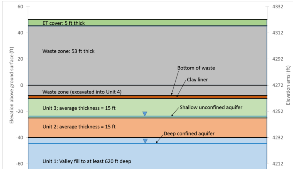
Figure 8. Hydrostratigraphic profile showing ET cover, waste zone, and hydrostratigraphy below the Federal DU Cell.
